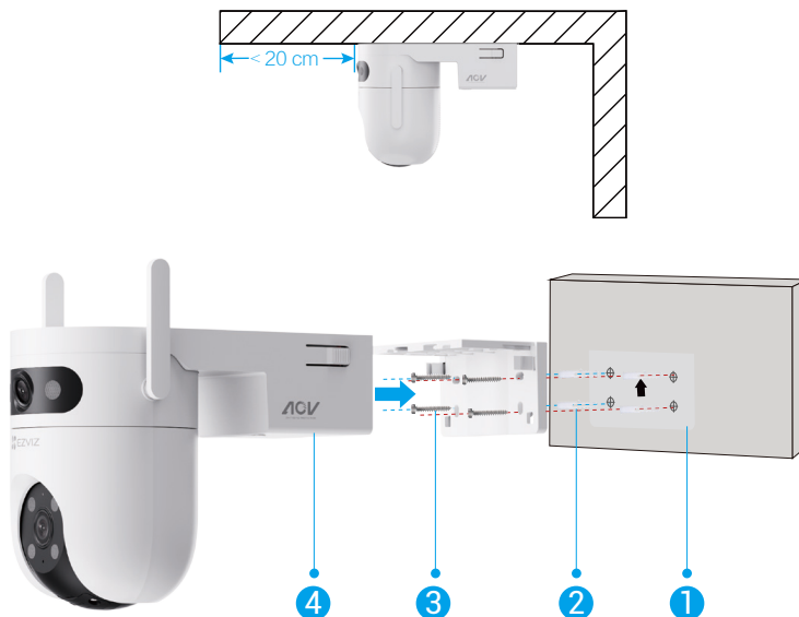
Fig. 2 Wall Mount
